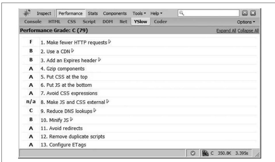
Figure 15-3. YSlow
