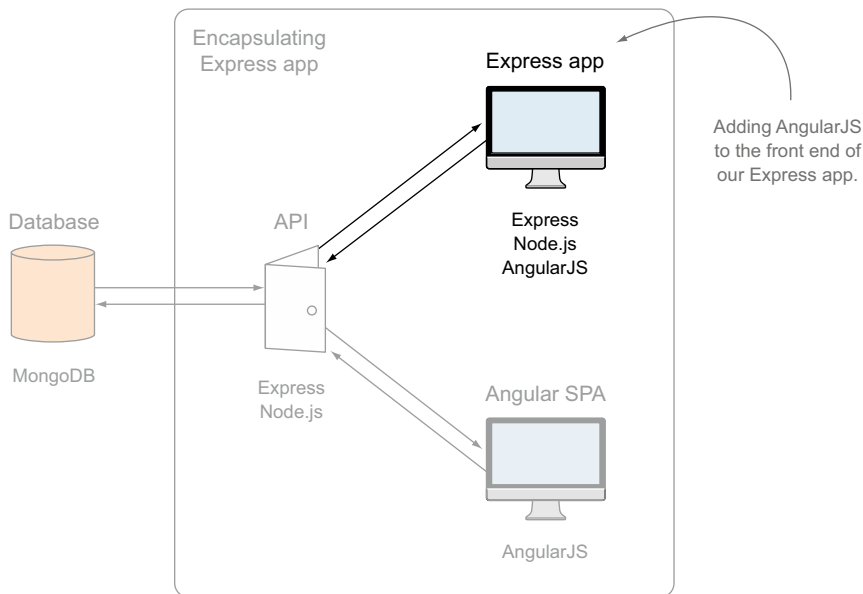
Figure 8.1 Chapter 8 focuses on adding Angular to the front end of the existing Express application.
