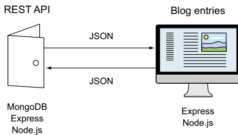
Figure 2.4 An architecture for delivering HTML directly from the server: an Express and Node.js application at the front, interacting with a REST API built in MongoDB, Express, and Node.js
