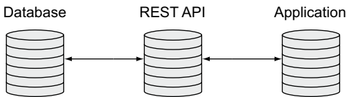
Figure 2.24 A decoupled architecture using three servers: one for the database, one for the API, and one for the application code
