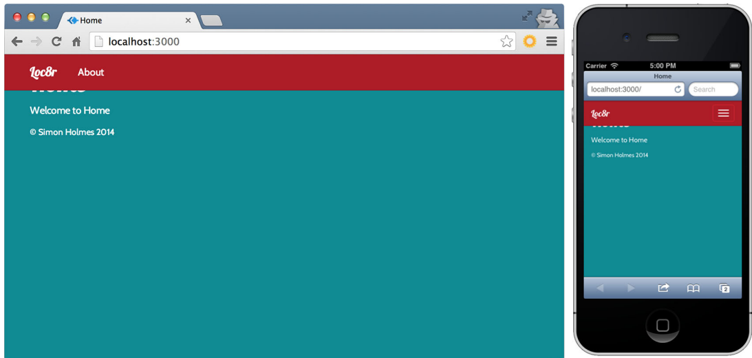
Figure 4.7 The homepage after the layout template has been set up. Bootstrap has automatically collapsed the navigation on the small screen size of the phone. The navigation bar overlaps the content, but that will be fixed when the content layouts are created.
