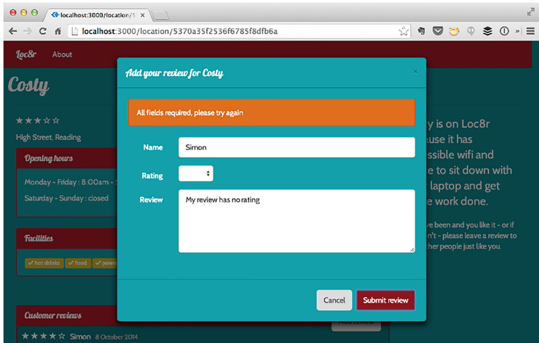
Figure 10.12 When an incomplete form is submitted, an error message is displayed.
