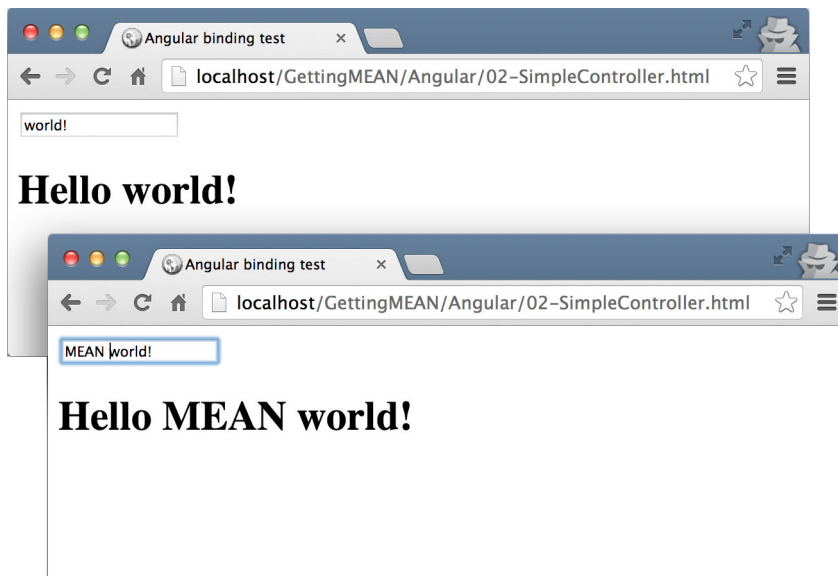
Figure 8.4 The controller assigns a default value via the scope, but we can still change that value using the input.
