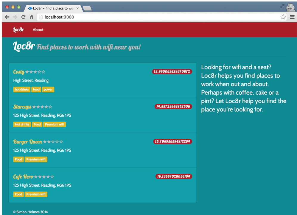
Figure 7.2 The first look at using data from the database in the browser—it's pretty close!
