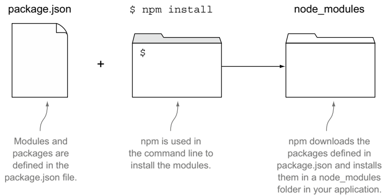
Figure 3.2 The npm modules defined in a package.json file are downloaded and installed into the application’s node_modules folder when you run the npm install terminal command.
