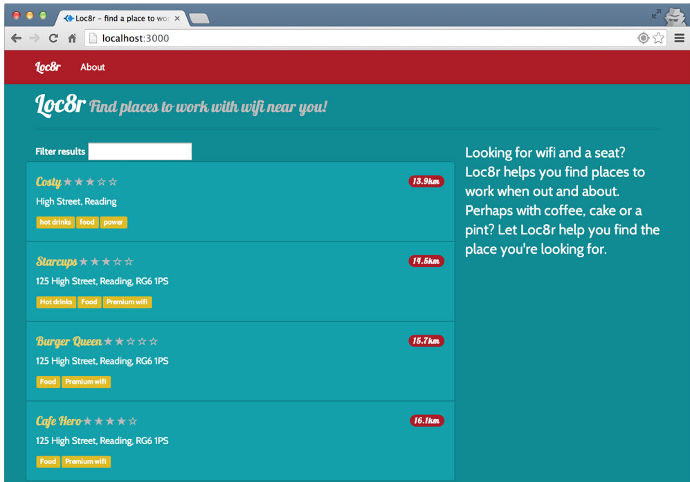
Figure 8.10 Visually the only difference to the homepage from the start of the chapter is the addition of the filter textbox; under the hood, however, the main content area is now being generated by Angular, which is also finding your actual location and displaying results close by.
