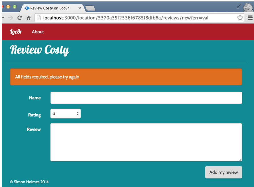
Figure 7.13 The validation error message showing in the browser, the end result of a process kicked off by Mongoose catching the error and returning it
