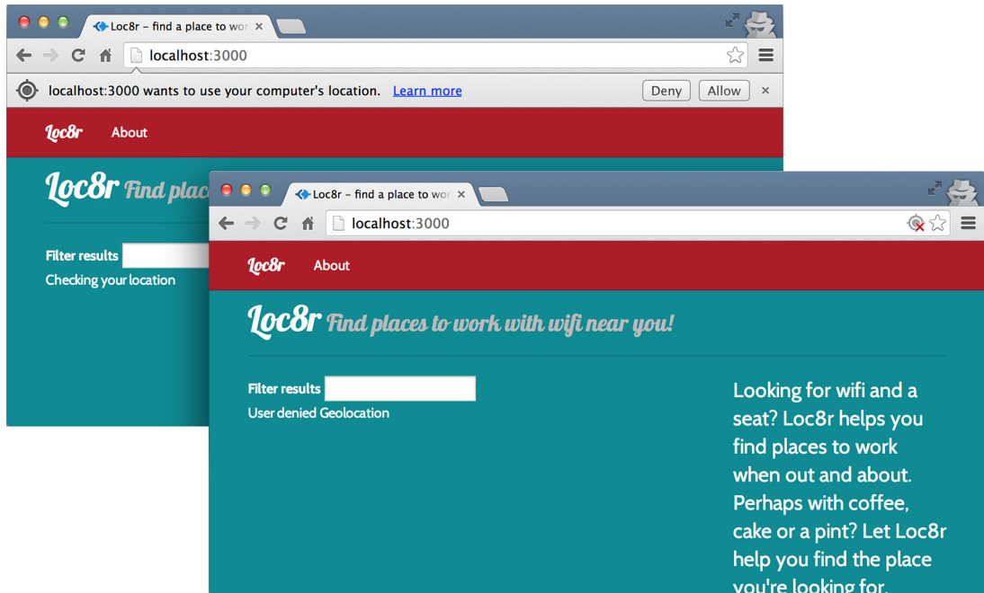
Figure 8.9 With geolocation added Loc8r will now ask your permission to know your location; if you say no then a simple message is displayed.
