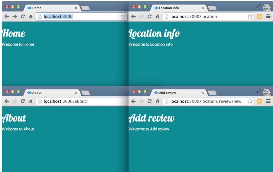
Figure 4.4 Screenshots of the four routes created so far, with different heading text coming through from the specific controllers associated with each route
