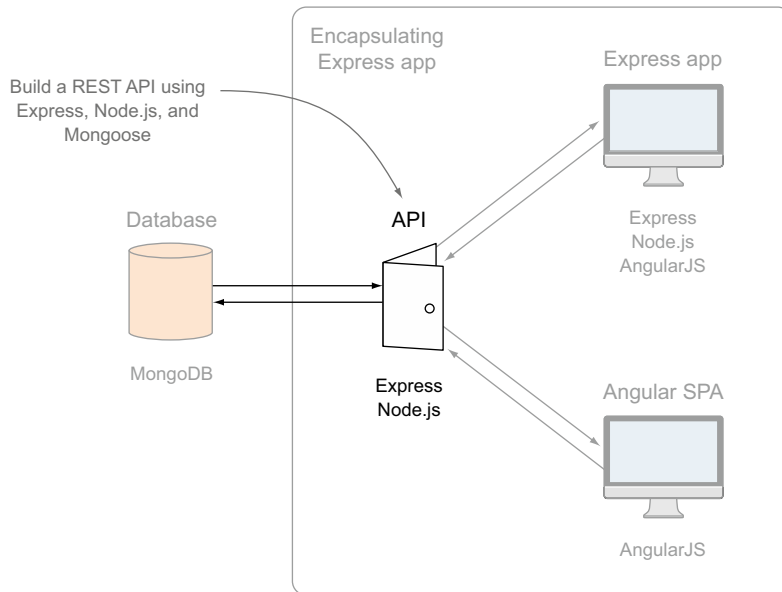
Figure 6.1 This chapter will focus on building the API that will interact with the database, exposing an interface for the applications to talk to.
