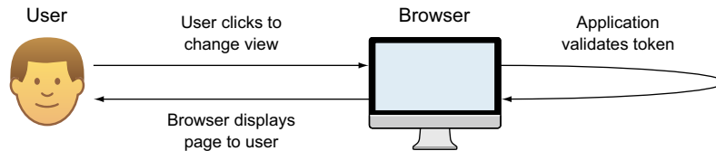
Figure 11.6 Using data inside the JWT, the SPA can determine which resources users can use or see.
