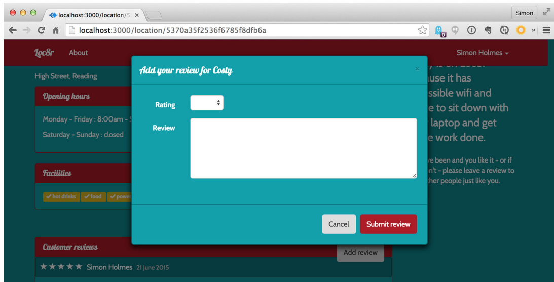
Figure 11.14 The final review form without a name field. Note the user's name in the top right and the logged-in version of the Add Review button.
