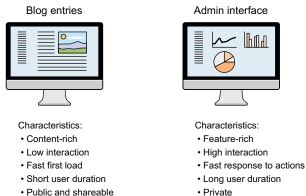
Figure 2.2 Conflicting characteristics of the two sides of a blog engine, the public-facing blog entries and the private admin interface
