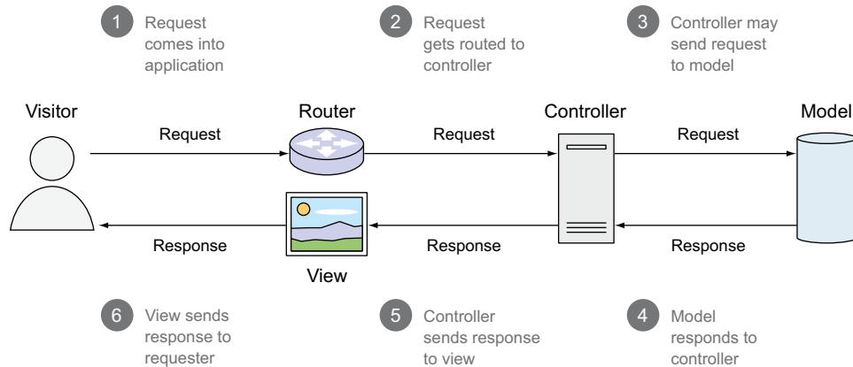
Figure 3.5 Request–response flow of a basic MVC architecture
