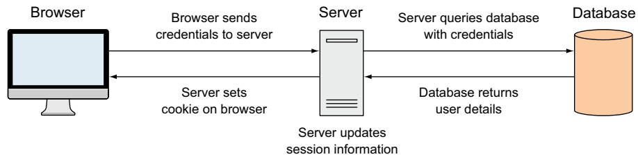
Figure 11.2 In a traditional server application the server and database validate user credentials and add them to users' sessions on the server.
