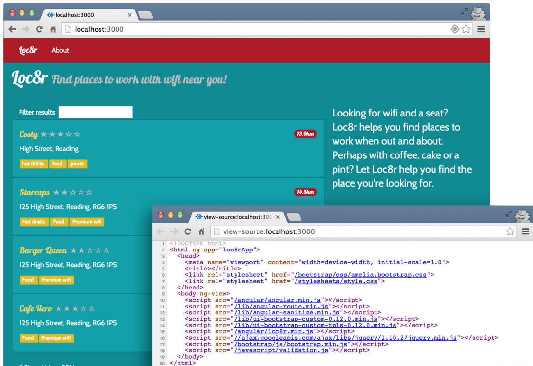
Figure 10.2 Now a real SPA, the source of the HTML page is minimal but the application is still fully functional.
