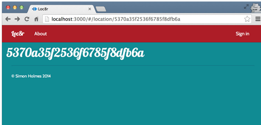
Figure 10.6 Using $routeParams we can get the location ID from the URL and use it in a controller, shown here by outputting it in the page header.
