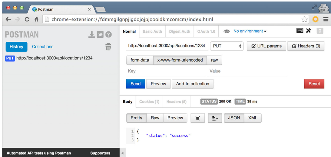
Figure 6.6 Using the Postman REST Client in Chrome to test a PUT request to the API
