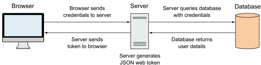
Figure 11.5 The login flow in a MEAN application, returning a JSON Web Token to the browser after the server validates user credentials
