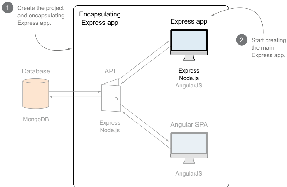
Figure 3.1 Creating the encapsulating Express application, and starting to set up the main Express application
