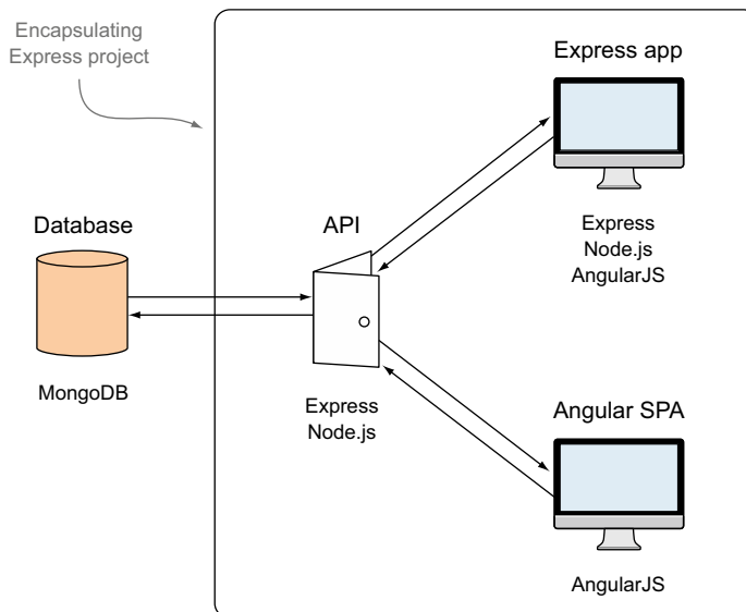
Figure 2.12 The architecture of the application with the API and application logic wrapped inside the same Express project
