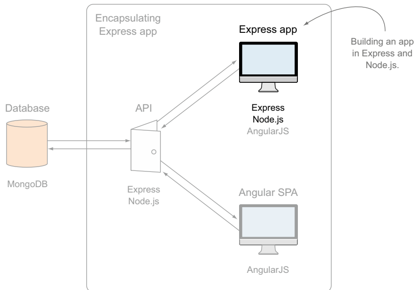
Figure 4.1 Using Express and Node to build a static site for testing views
