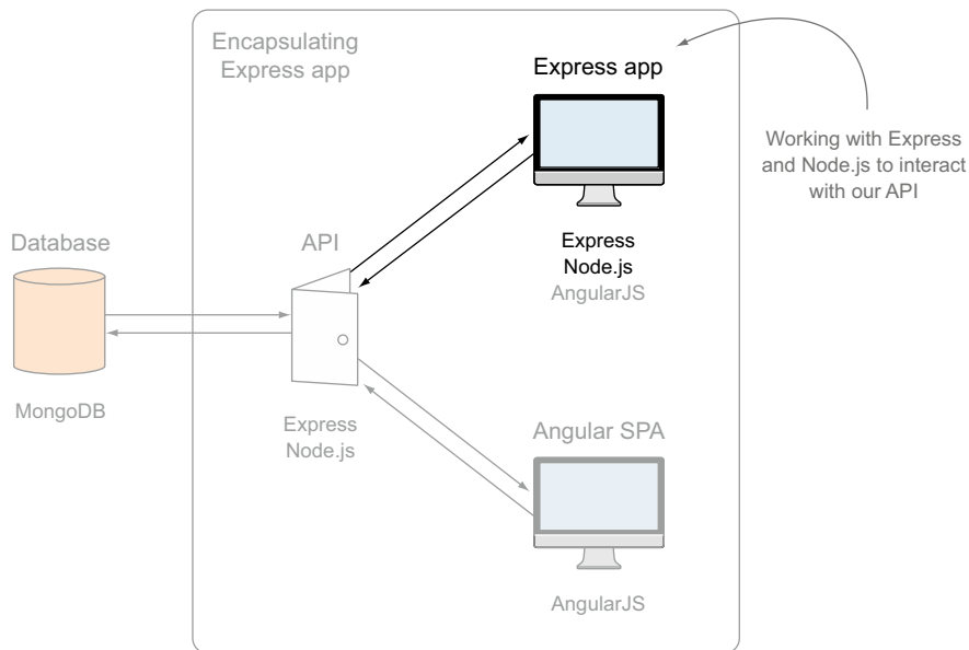
Figure 7.1 This chapter will focus on updating the Express application from chapter 4 to interact with the REST API developed in chapter 6.
