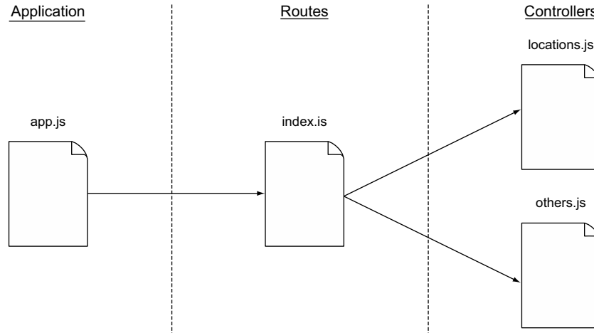
Figure 4.3 Proposed file architecture for routes and controllers in our application
