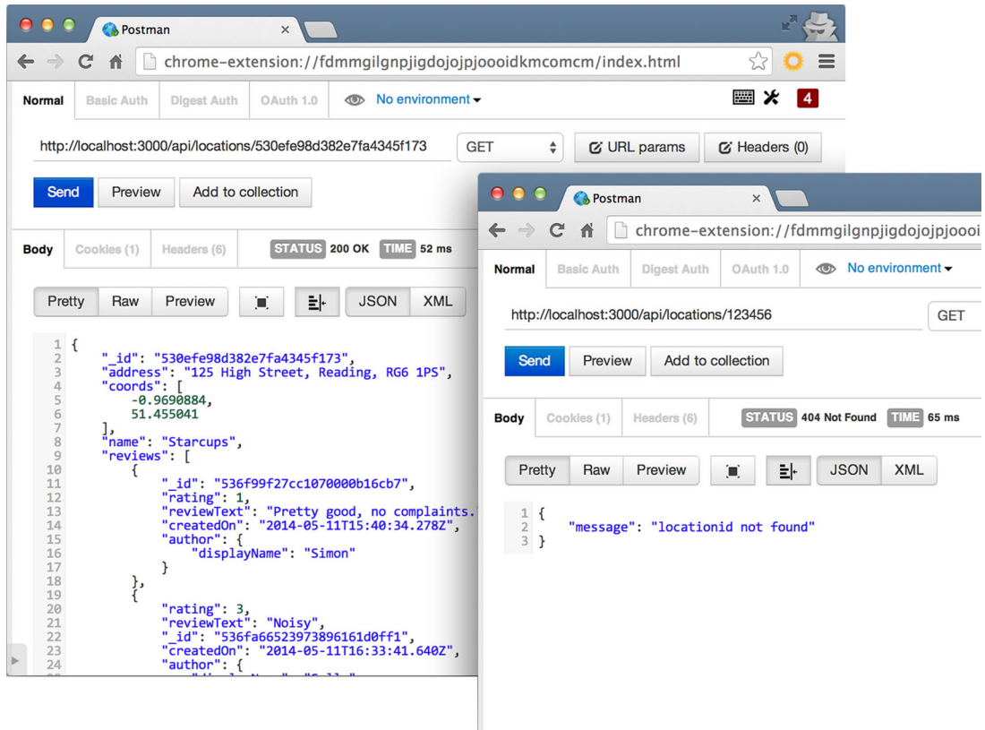
Figure 6.8 Testing successful (left) and failed (right) API responses using Postman
