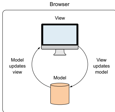
Figure 8.2 In Angular the view and model are bound together with two-way data binding, all in the browser.
