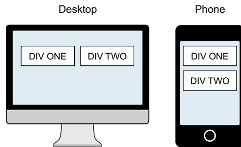
Figure 4.5 Bootstrap's responsive column system on a desktop and mobile device. CSS classes are used to determine the number of columns out of 12 that each element should take up at different screen resolutions.
