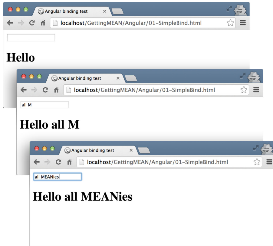
Figure 8.3 With simple data binding in Angular, as soon as text is typed into the input box it's output inside the <h1> tag. This is all achieved without having to write a single line of code.
