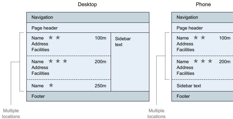
Figure 4.8 Desktop and mobile layout sketches for the homepage. Sketching out the layouts for a page can give you a quick idea of what you’re going to build, without getting distracted by the intricacies of Photoshop or technicalities of code.
