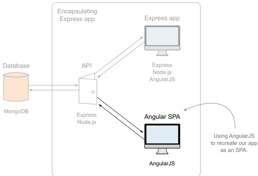
Figure 9.1 This chapter will recreate the Loc8r application as an Angular SPA, moving the application logic from the back end to the front end.
