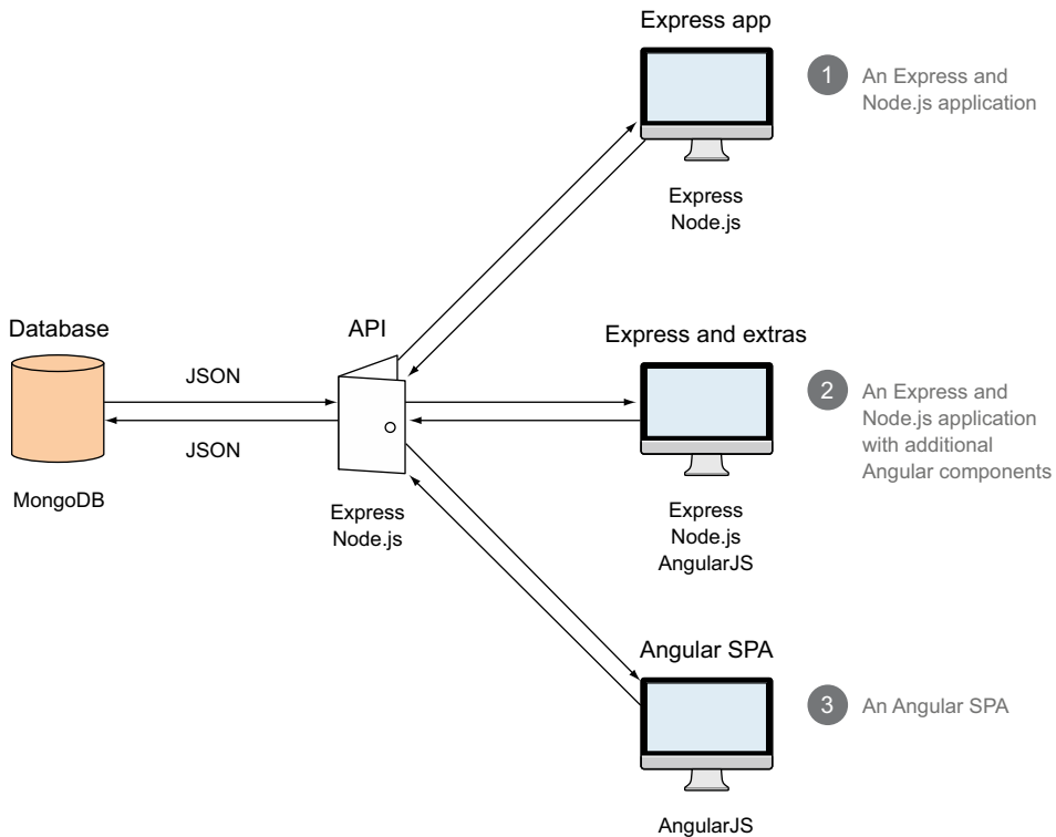
Figure 2.11 Three options for building the Loc8r application, ranging from a server-side Express and Node.js application to a full client-side AngularJS SPA
