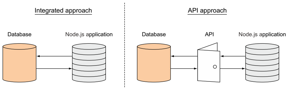
Figure 2.7 The short-term view of data integration into your Node.js application. You can set up your Node.js application to talk directly to your database, or you can create an API that interacts with the database and have your Node.js application talk only with the API.
