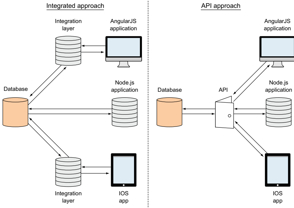
Figure 2.8 The long-term view of data integration into your Node.js application, and additional AngularJS and iOS applications. The integrated approach has now become fragmented, whereas the API approach is simple and maintainable.
