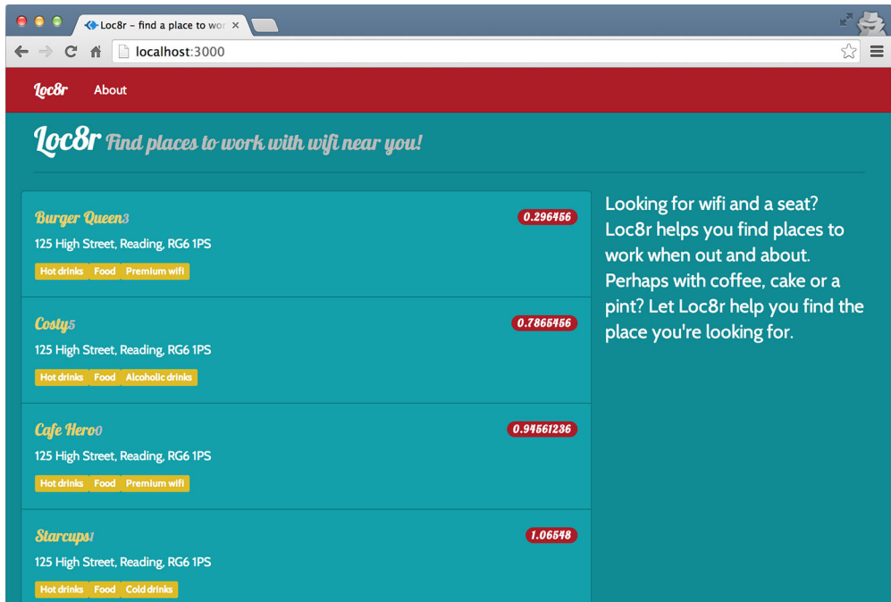
Figure 8.5 The homepage data being supplied and rendered by Angular instead of Express. There are some layout issues that need fixing.
