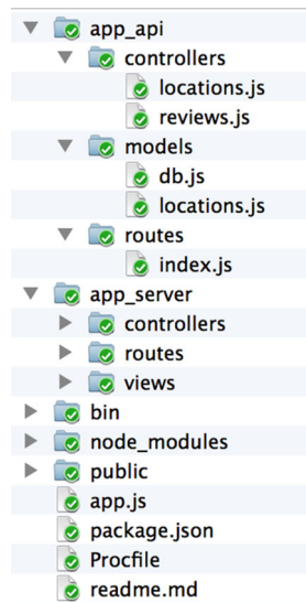
Figure 6.4 Folder structure of the application at this point: app_api has models , controllers , and routes , and app_server has views , controllers , and routes
