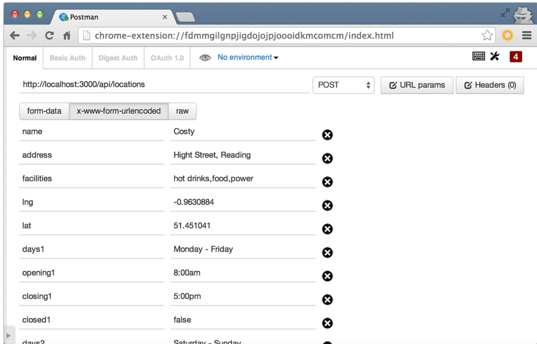
Figure 6.11 Testing a POST method in Postman, ensuring that the method and form data settings are correct
