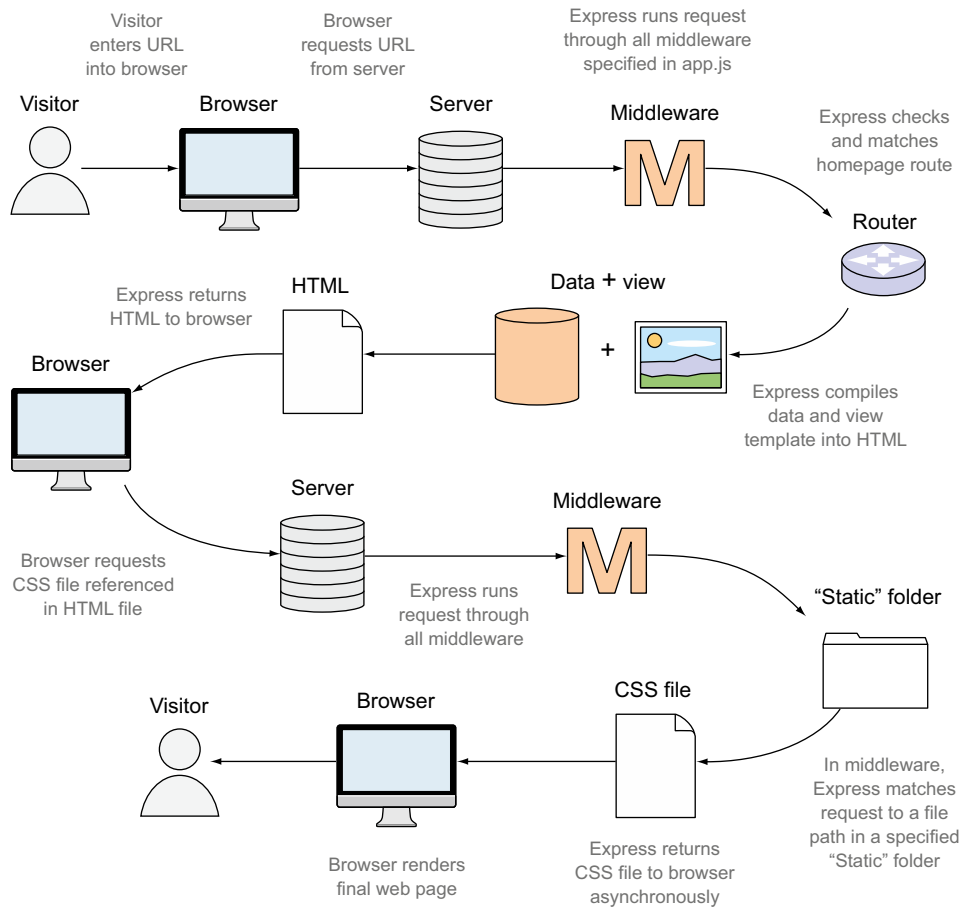
Figure 3.4 The key interactions and processes that Express goes through when responding to the request for the default landing page. The HTML page is processed by Node to compile data and a view template, and the CSS file is served asynchronously from a static folder.
