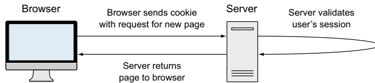
Figure 11.3 In a traditional server application the server validates users' sessions before continuing with a secure request.
