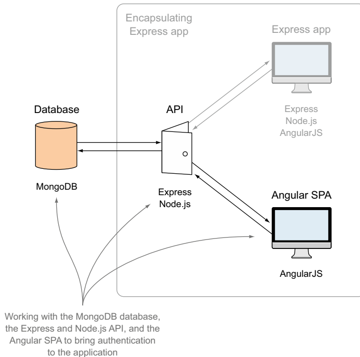
Figure 11.1 This chapter adds an authentication system to the application that touches most parts of the architecture, such as the database, API, and front-end SPA.
