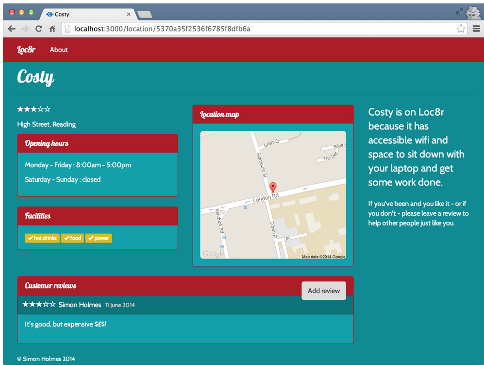
Figure 7.8 The complete Details page. The ID of the location is passed from the URL to the API, and the API retrieves the data and passes it back to the page to be formatted and rendered correctly.
