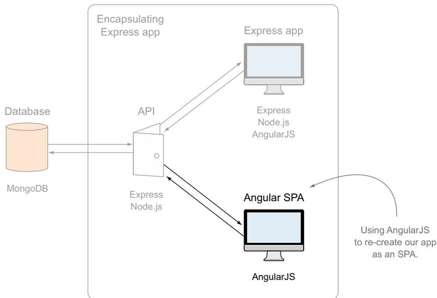
Figure 10.1 This chapter continues the work we started in chapter 9 of re-creating the Loc8r application as an Angular SPA, moving the application logic from the back end to the front end.
