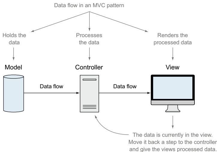
Figure 4.14 How the data should flow in an MVC pattern, from the model through the controller to the view. At this point in the prototype our data is in the view, but we want to move it a step back into the controller.
