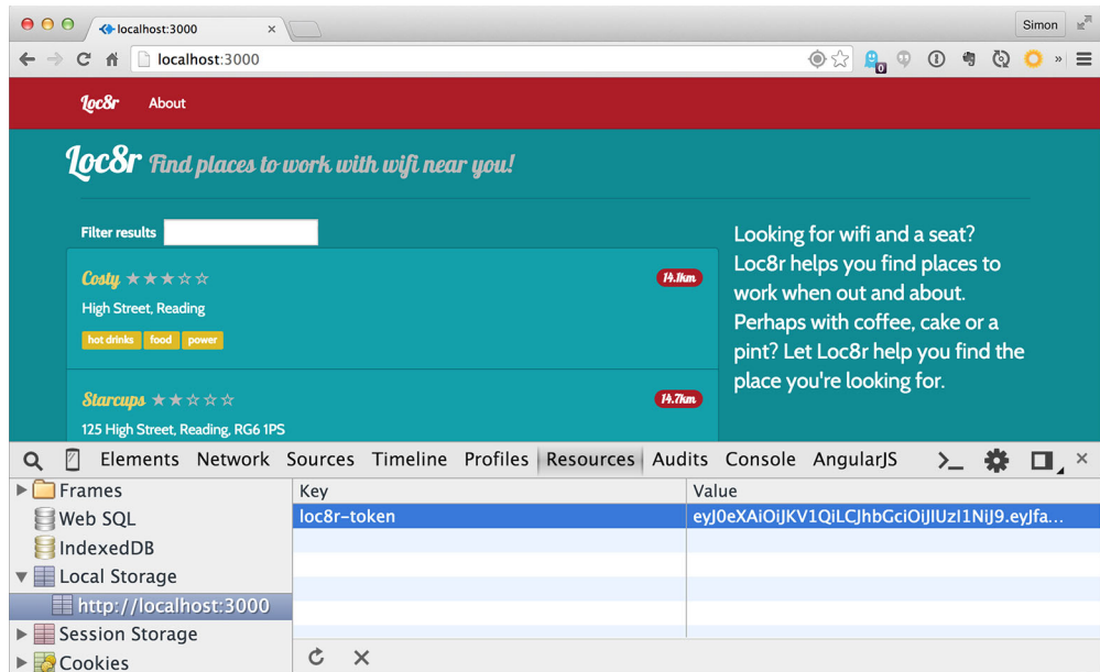
Figure 11.12 Finding the loc8r-token in the browser
