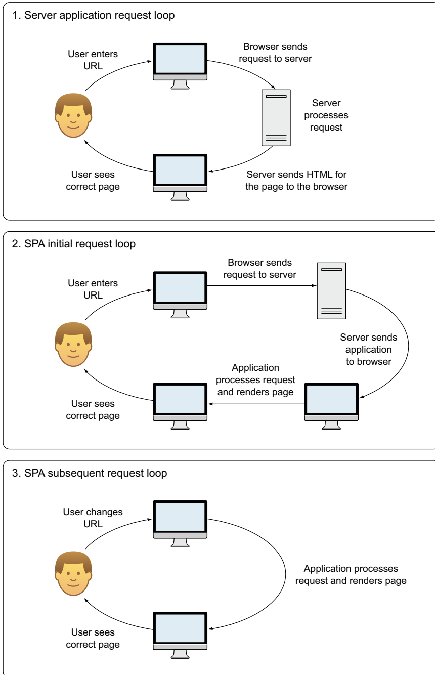
Figure 9.2 Three different request loops associated with different approaches. Server applications hit the server for every new page request, but SPAs typically only hit the server for the initial page load. Subsequent requests are handled by the SPA itself.
