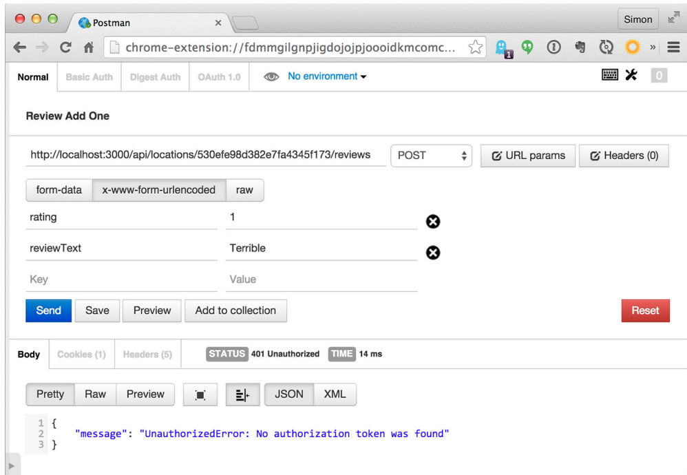
Figure 11.11 Trying to add a review without a valid JWT now results in a 401 response.
