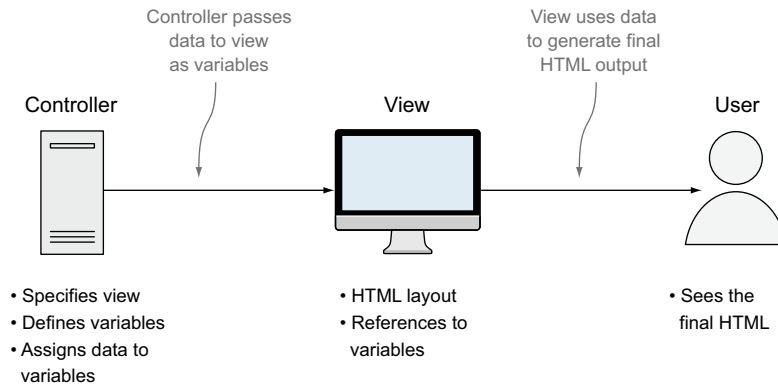
Figure 4.15 When the controller specifies the data, it passes the data to the view as variables; the view then uses that data to generate the final HTML that's delivered to the user.
