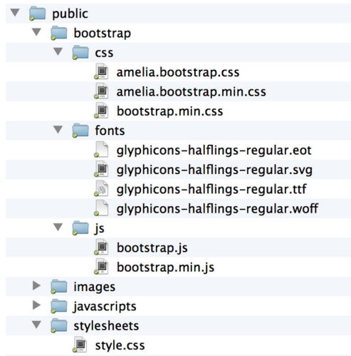
Figure 3.8 Structure of the public folder in the Express application after adding Bootstrap
