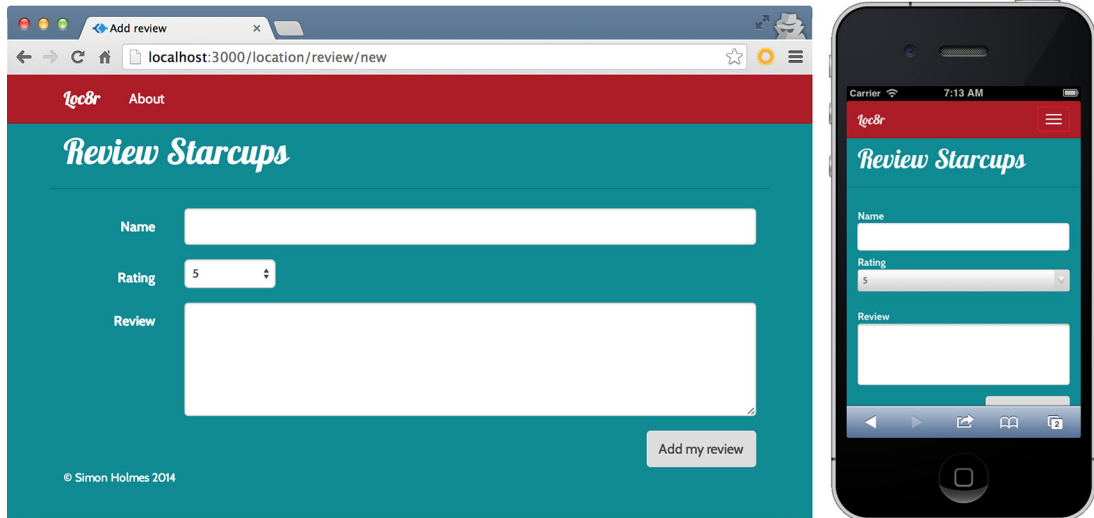
Figure 4.12 Complete Add Review page in a desktop and mobile view
