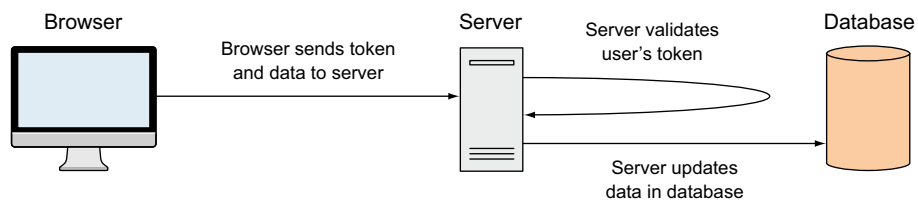
Figure 11.7 When calling an authenticated API endpoint, the browser sends the JWT along with the data; the server decodes the token to validate a user's request.
