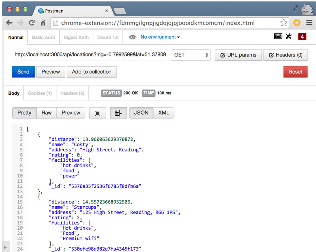
Figure 6.10 Testing the location list route in Postman should give a 200 status and a list of results, depending on the geographical coordinates sent in the query string.
