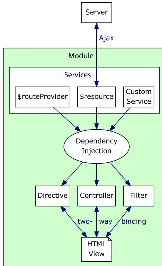
Figure 9—Overview of some AngularJS concepts
