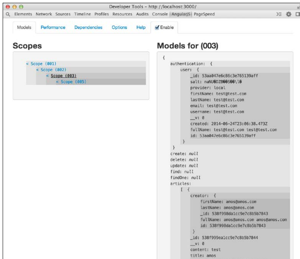
Batarang models
