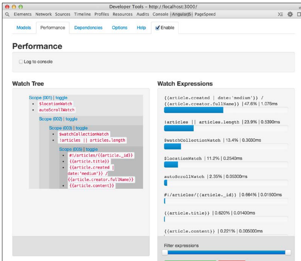
Batarang performance
