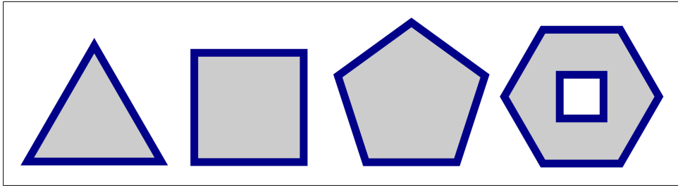
Figure 21-6. Regular polygons
